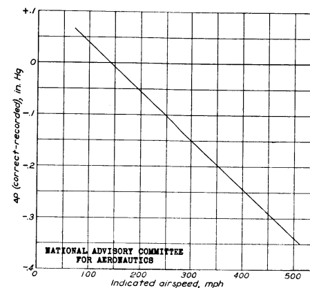
Figure 4.- Recorded static position-error correction, North American P-51B-1-NA airplane.
