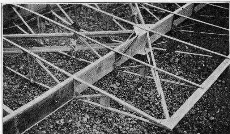
Plate XXI. Detail of Prüfling Wing Showing Aileron Hinge and Rear Strut Attachment
