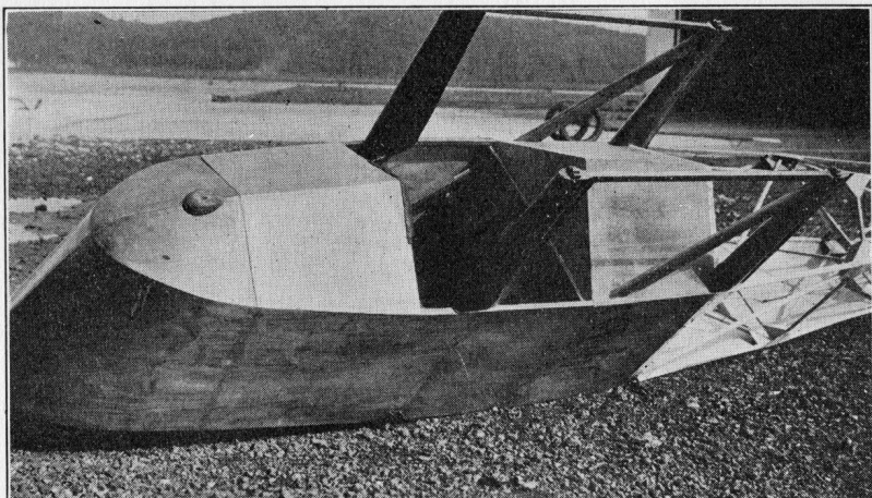
Plate XXXIX. The Prüfling Fuselage, Showing the Removable Cowl Cover in Place, and the Center Section Struts
