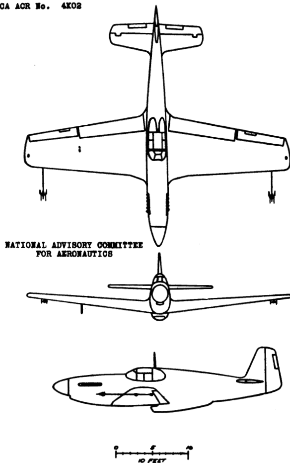
FIGURE 1.—THREE-VIEW DRAWING OF THE NORTH AMERICAN P-51B-1-NA AIRPLANE.
