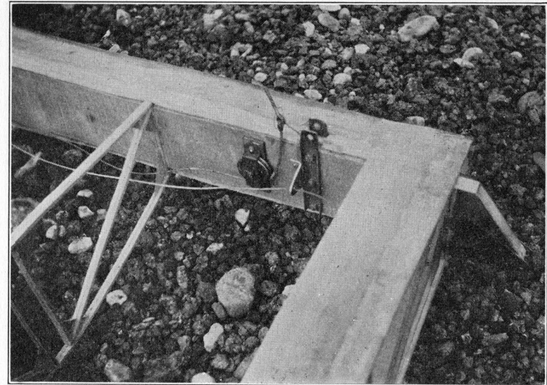
Plate XXVI. Center Section Strut Attachment Fitting and Aileron Pulley in Prüfling Wing
