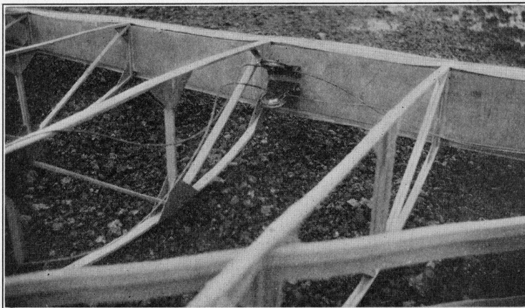
Plate XXV. Aileron Pulleys in Prüfling Wing
