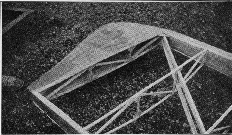
Plate XXIV. Prüfling Wing Tip
