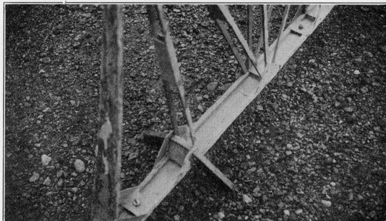
Plate XXXI. Detail of Prüfling Rudder Showing Control-Horn Attachment
