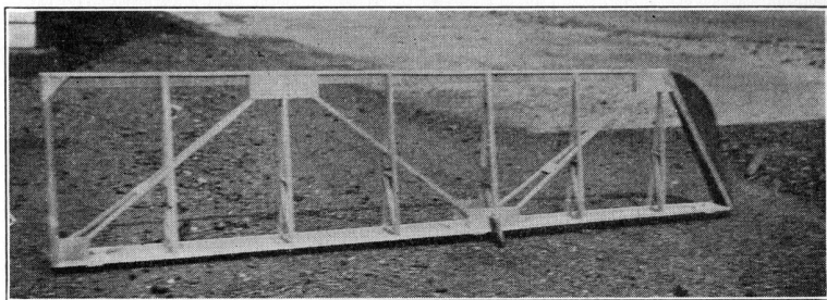
Plate XXVIII. Prüfling Aileron
