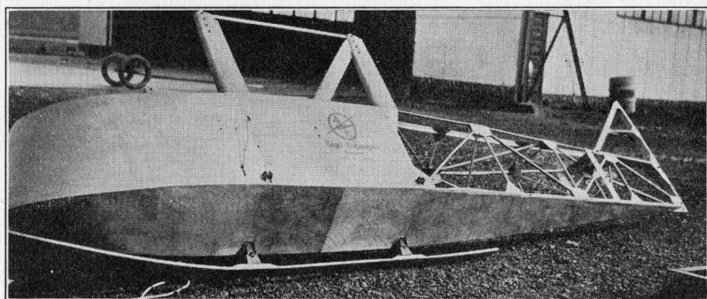
Plate XL. The Bottom of the Prüfling Fuselage, Showing the Attachment of the Skid
