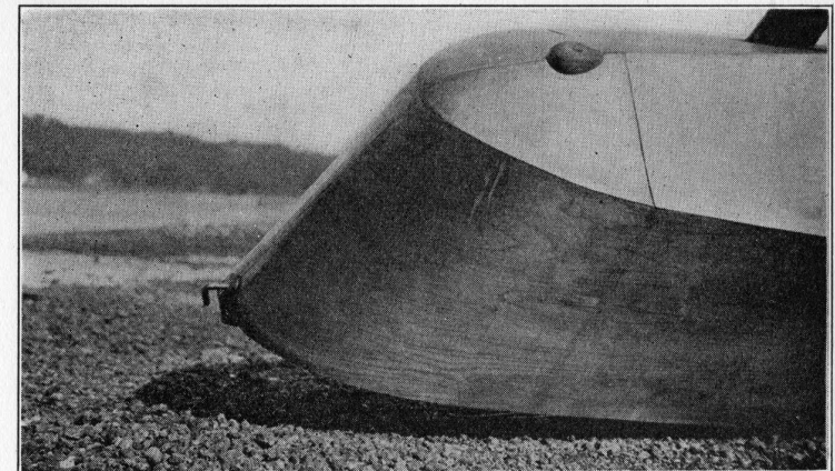
Plate XXXVIII. The Nose of the Prüfling Fuselage, Showing Towing Hook
