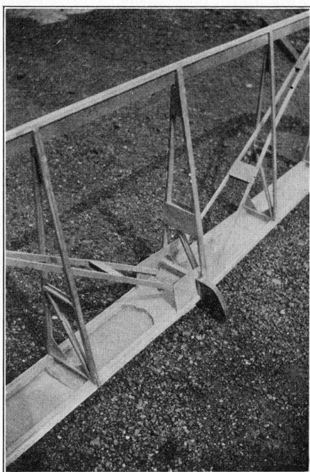
Plate XXIX. Detail of Prüfling Aileron Showing Control Horn
