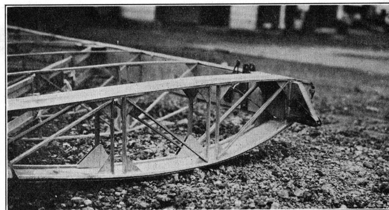
Plate XXIII. Prüfling Front Wing Hinge
