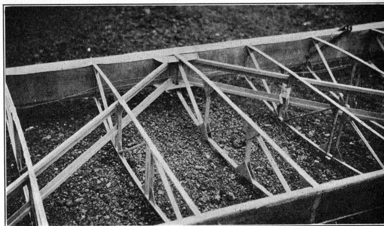
Plate XXII. Detail of Prüfling Drag Bracing
